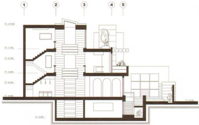
Cross section
